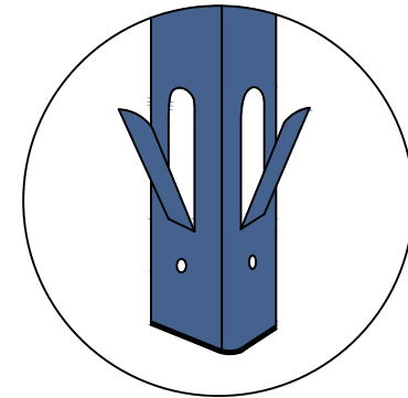
PATENTED ANCHOR DETAIL ISOMETRIC VIEW N.T.S
